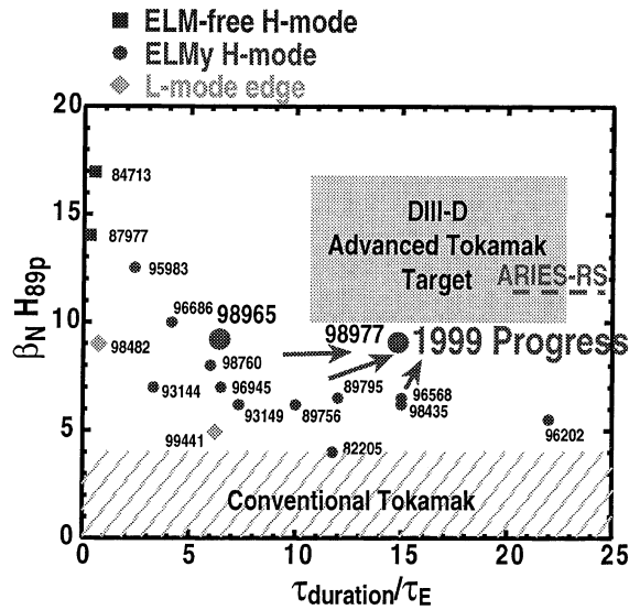
Fig. 1. A plot of the \beta_N H product as a function of \tau_{\text{duration}}/\tau_E for several types of DIII-D discharges with ohmic and NBI current profile control. ELM-free H -modes have good confinement but have been limited to short duration. The ELMing H -mode has achieved the best performance so far; recent discharges (98977 and 98965) are highlighted. The shaded box represents an AT target, and typical parameters of the ARIES-RS reactor design are included.
