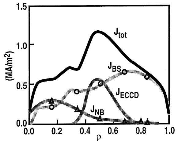
Fig. 2. Calculation of the required current profiles for a sustained ECCD AT scenario obtained from the ONETWO transport model. Note that for ECH power levels \sim 3 MW, the divertor must control the density in the range of 40% of the Greenwald density.
