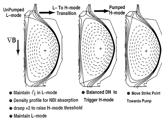
Fig. 5. One illustration of how plasma shape can control the particle exhaust and the H -mode power threshold. From left to right, the magnetic balance parameter D_{\text{rsep}} is +2 cm to raise the H -mode threshold in the beginning of the discharge to provide a peaked density profile for efficient beam penetration. The D_{\text{rsep}} is then set close to 0, magnetic balance, to trigger H -mode and increase the confinement. Shortly after this time, the strike point is swept towards the pump to maintain the target density for the ECCD portion of the discharge.
