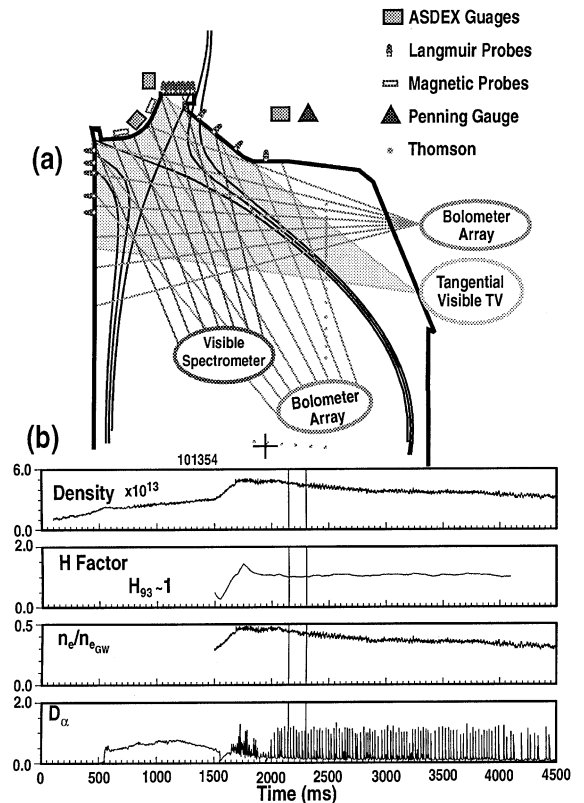
Fig. 4. Several new diagnostics have been installed with D-2000, including an array of Langmuir probes, ASDEX and Penning gauges, visible spectroscopy views, and a visible TV camera. D-2000 has been used to reduce the core electron density to 30–40% of the Greenwald density, which is sufficient for the AT scenarios with the current ECCD power on DIII-D.
